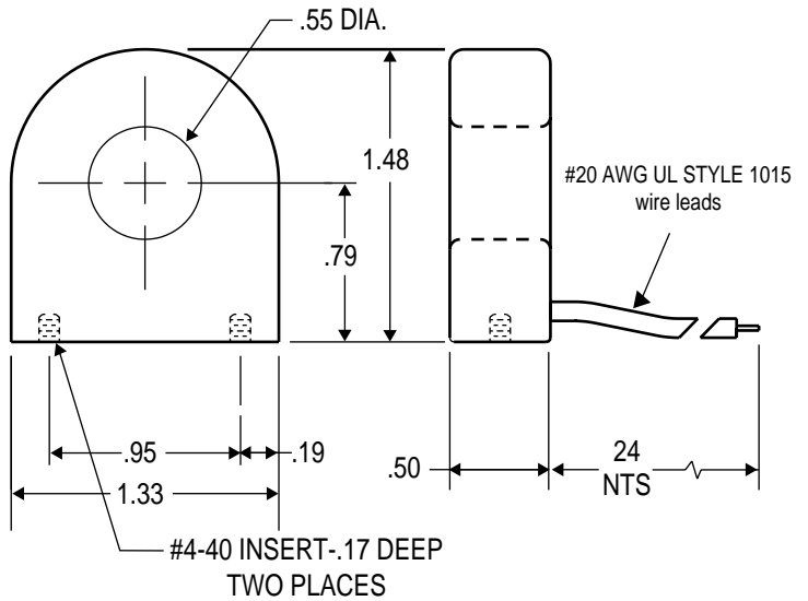
Model 17 & 18: Current Sensing Transformers
