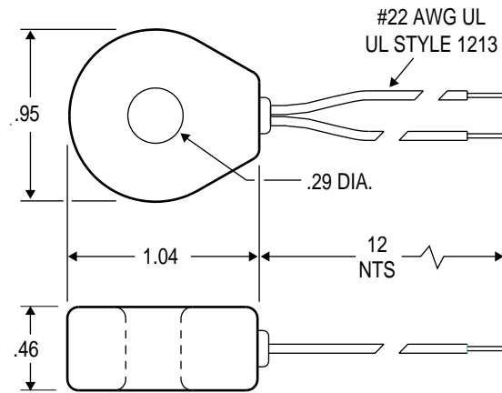
Model 19: Current Sensing Transformer
