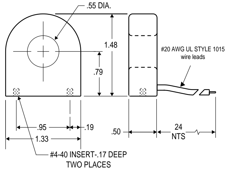
Model 17 & 18: Current Sensing Transformers
