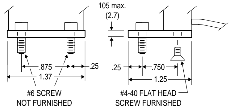
MB-18: Surface Mounting Bracket for Model 17 & Model 18
